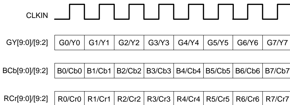
Figure 4–1. 24-/30-Bit RGB or YCbCr Data Format
